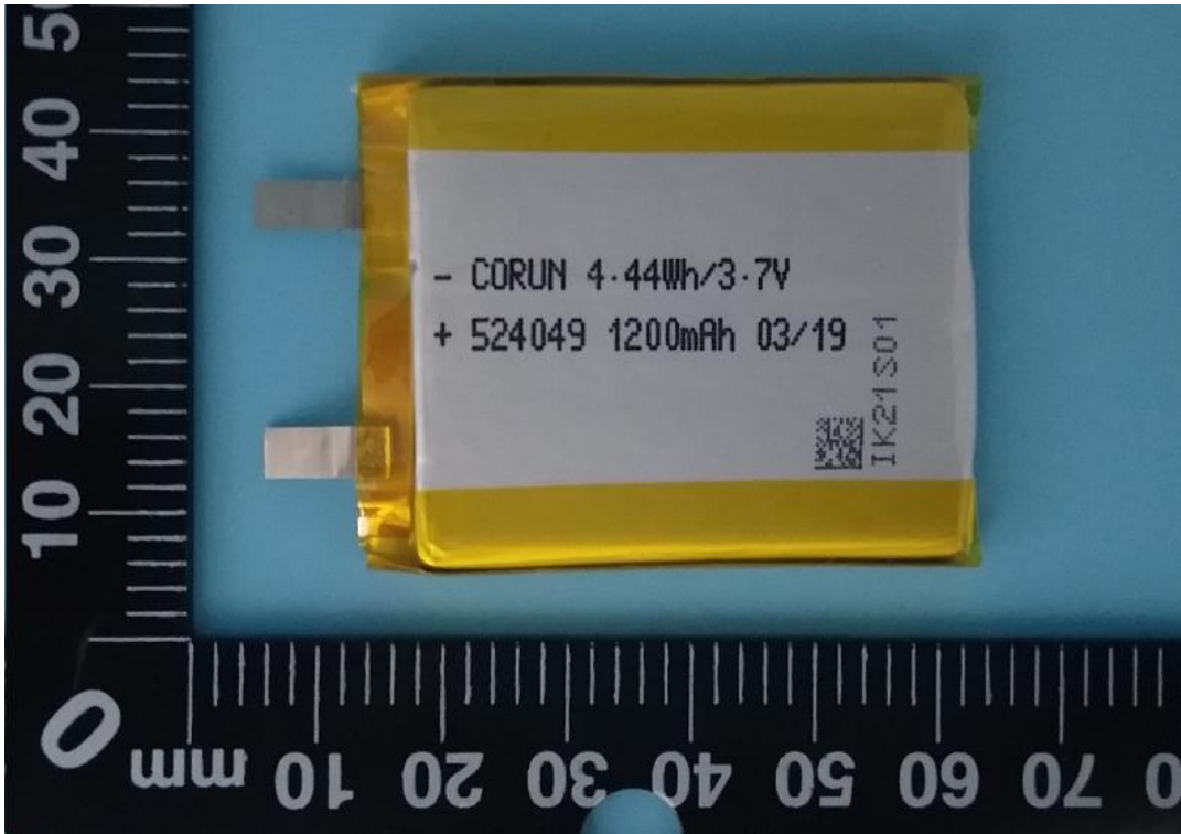
Cell /电芯 (524049 3.7V 1200mAh 4.44Wh)
