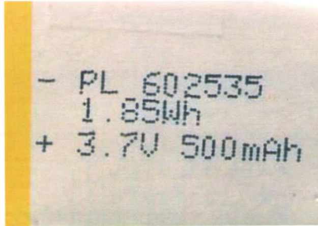
电池组铭牌 Battery Nameplate
