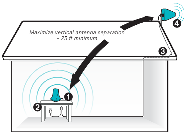
Installation overview
