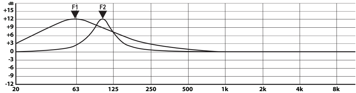
F1: 60Hz Center Frequency | 0.50 Q Factor F2: 100Hz Center Frequency | 2.00 Q Factor
