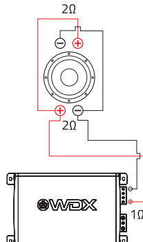
1 X 2Ω DVC SUBWOOFER
