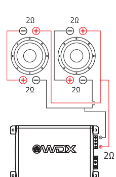
2 X 2Ω DVC SUBWOOFERS
