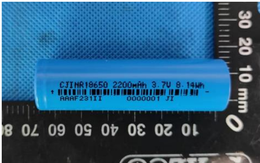
Photo 1 电池正面 Front view of Cell
